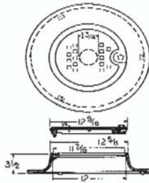
6150TR Meter Cover
