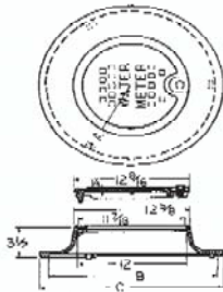
6150 Meter Box Cover
