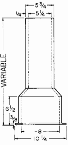
6855 Box
