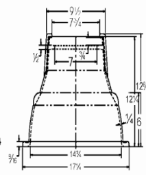
6860 #6 Base
