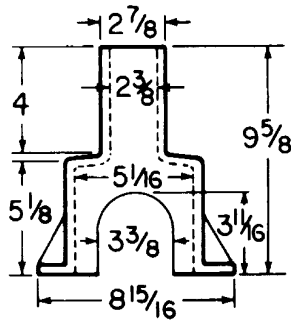
ENLARGED BASE For 2" Curbstops
